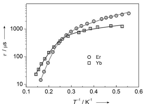
Figure 3. Temperature dependence of the relaxation time ( \tau in \mu\text{s} ) for Er and Yb derivatives in static field 1000 Oe. The solid lines correspond to the best fit assuming a combination of exponential and power law dependences on T of the relaxation rate.
